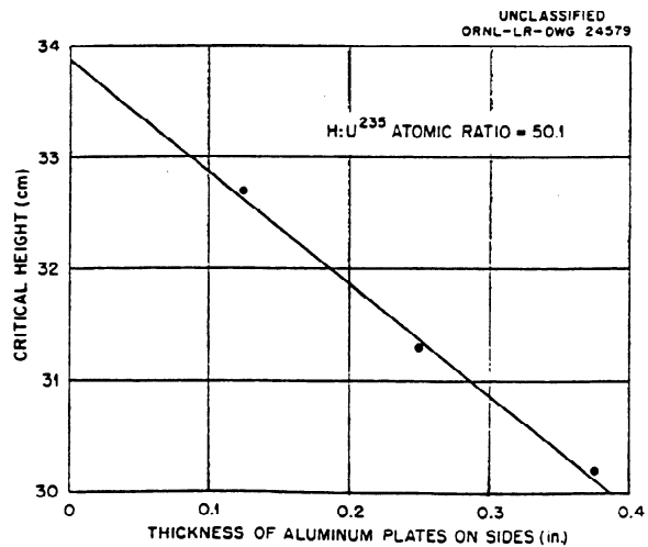
Fig. 4.1.4. Critical Height of a 6-in.-Thick Slab of Enriched U 235 Solution Contained in an Aluminum Vessel as a Function of the Thickness of Aluminum on the Two Faces of the Slab.
