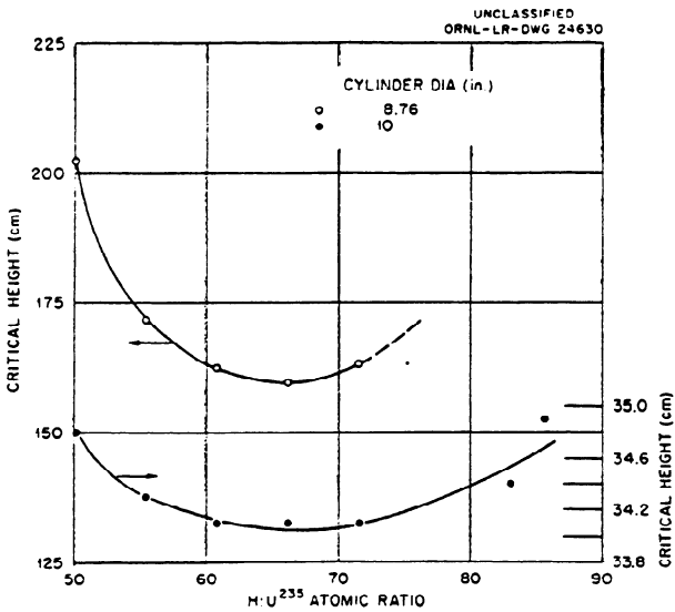
Fig. 4.1.2. Critical Height of Unreflected Enriched U 235 Solutions Contained in Aluminum Cylinders as a Function of the H:U 235 Atomic Ratio of the Solutions. Ratios from 50 to 86.
