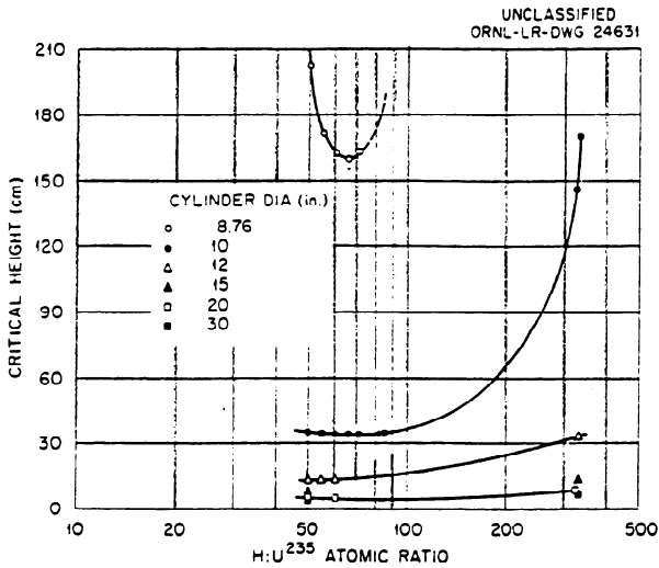
Fig. 4.1.1. Critical Height of Unreflected Enriched U 235 Solutions Contained in Aluminum Cylinders as a Function of the H:U 235 Atomic Ratio of the Solutions.
