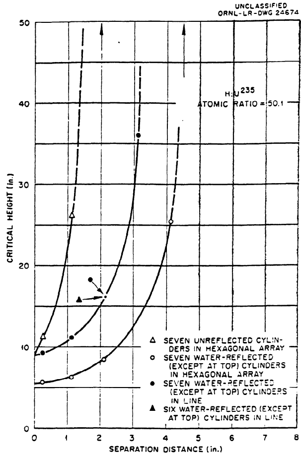
Fig. 4.1.15. Critical Height of Arrays of 5-in.-dia Cylinders Containing Enriched U 235 Solution.
